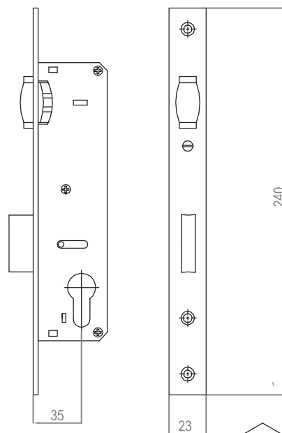
ART 155 35 20 pcs Mourtise lock with roller
