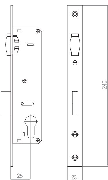
ART 155 25 20 pcs Mourtise lock with roller
