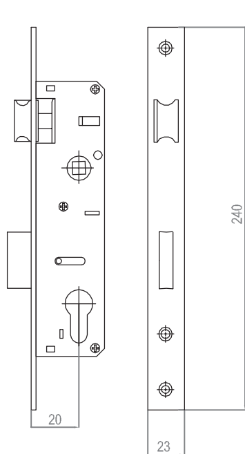
ART 153 20 30 pcs Mourtise lock with cylinder
