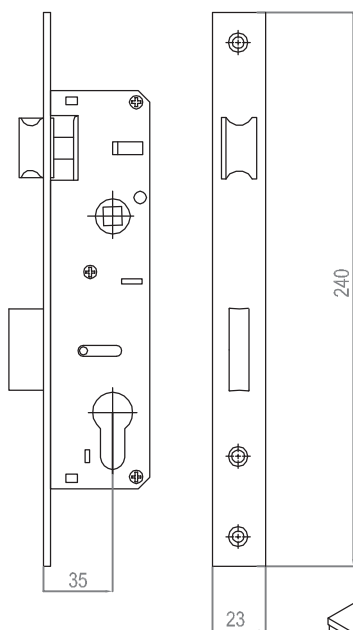
ART 153 35 20 pcs Mourtise lock with cylinder
