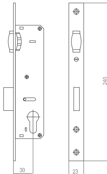
ART 155 30 20 pcs Mourtise lock with roller
