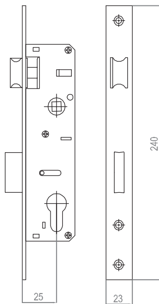
ART 153 25 20 pcs Mourtise lock with cylinder
