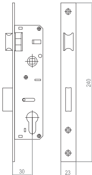
ART 155 30 30 pcs Mourtise lock with cylinder
